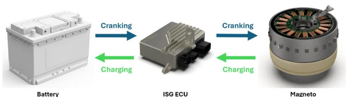
Energy Conversion in an ISG system Image source: SEDEMAC
